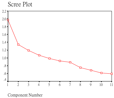
Figure 1. Scree Plot
