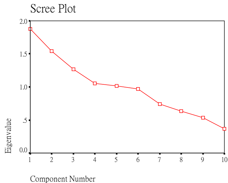
Figure 1: Scree plot
